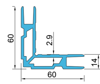
XFA-KEVP-04 T=2.9 mm W=1.77 Kg/m
